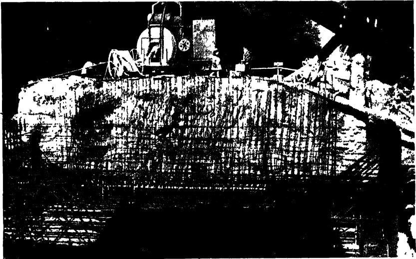
Fig. 188. —Reinforcement in Abutment, Dinnet Bridge.
